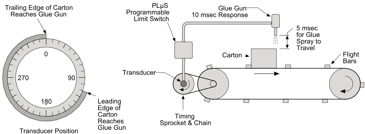
Figure 25—Speed Compensation at Various Speeds
