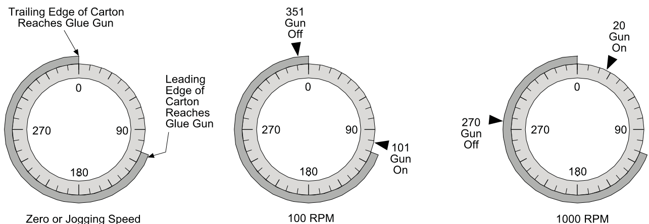
Figure 25—Speed Compensation at Various Speeds
