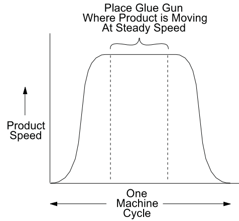
Figure 29—Product Speed Should be Constant Past Controlled Device
