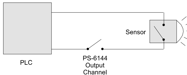
Figure 26—Simple Sensor Gating Scheme
